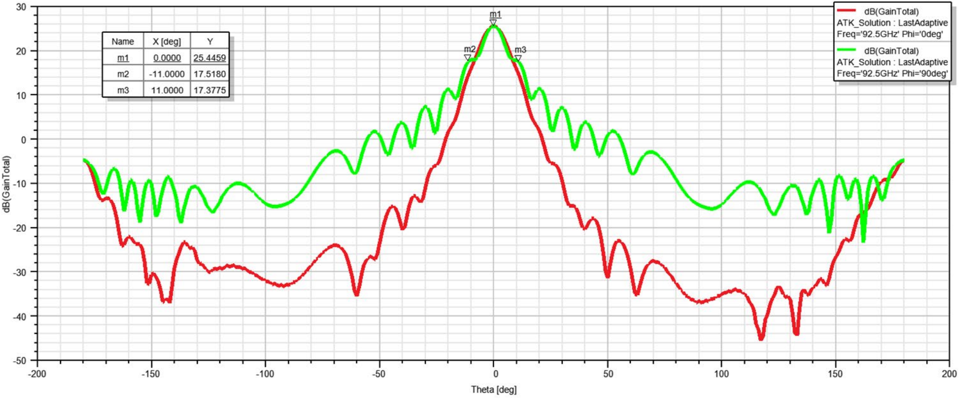
Beamwidth Pattern @ 92.5 GHz
