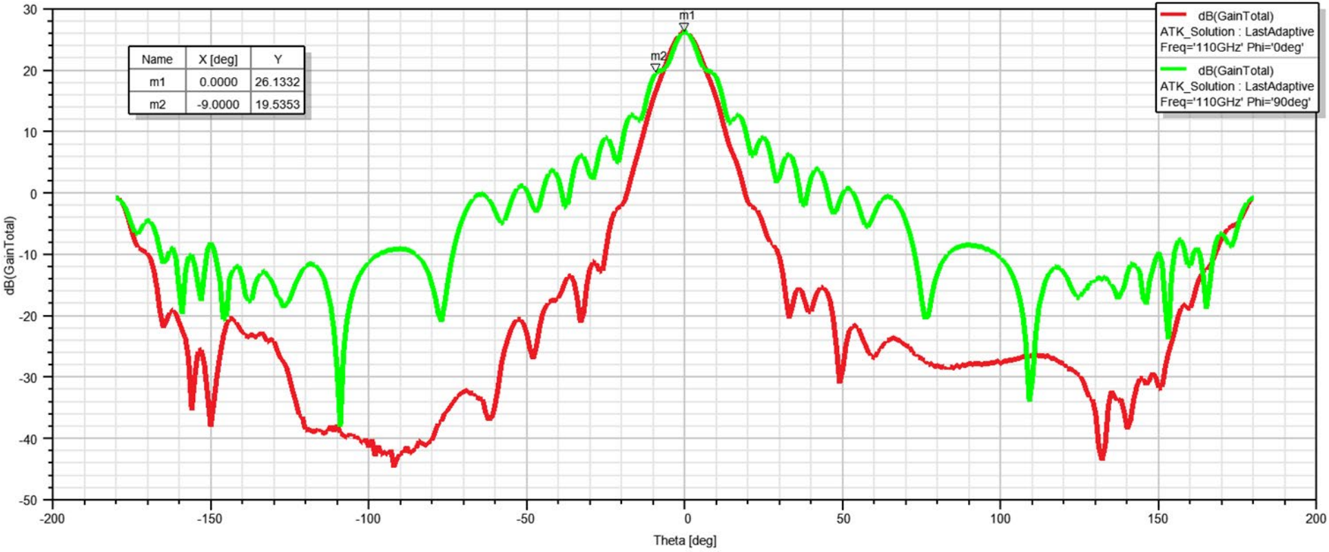
Beamwidth pattern @ 110 GHz
