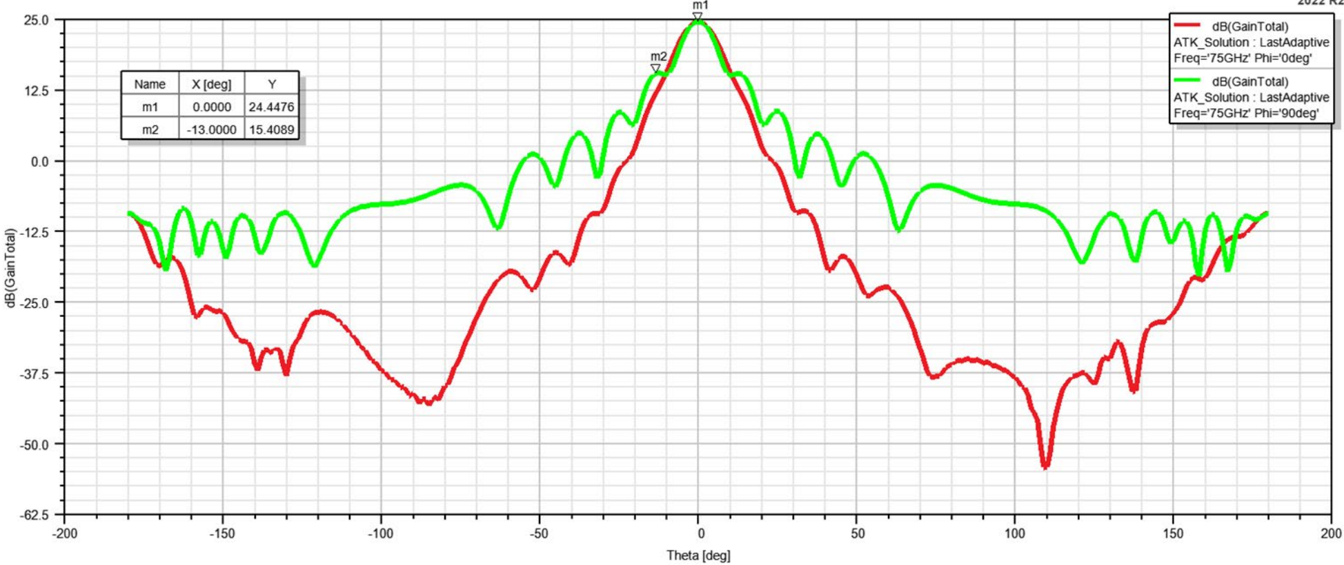
Beamwidth pattern @ 75 GHz
