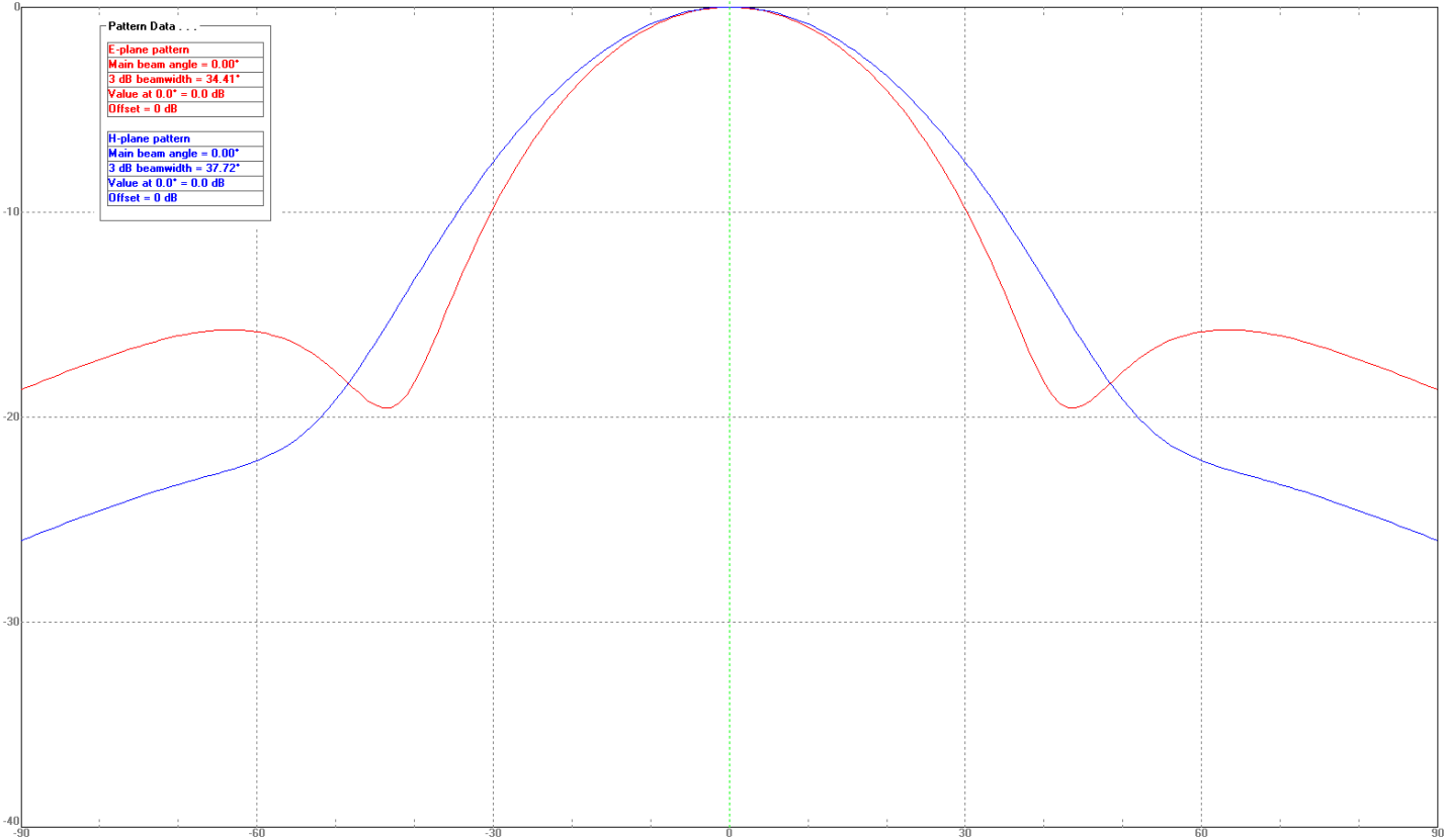
Beamwidth Pattern at 26.5 GHz
