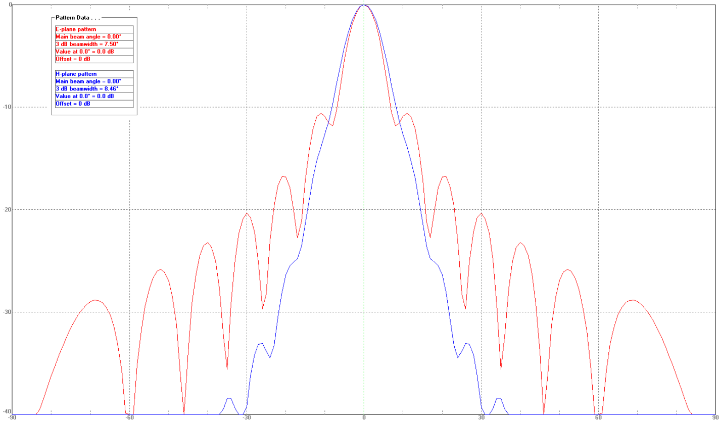
Beamwidth Pattern at 260 GHz
