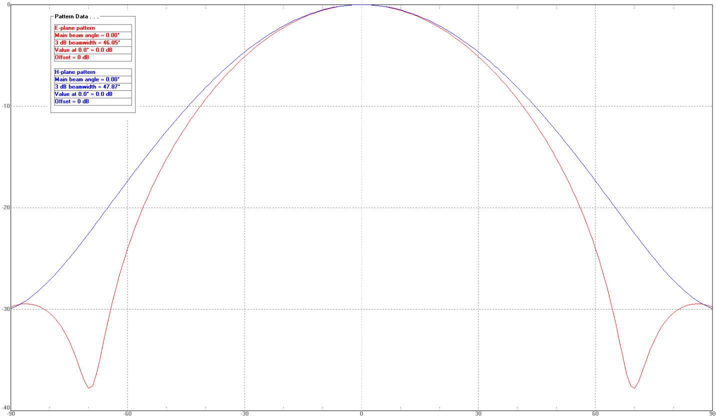
Beamwidth Pattern at 90 GHz
