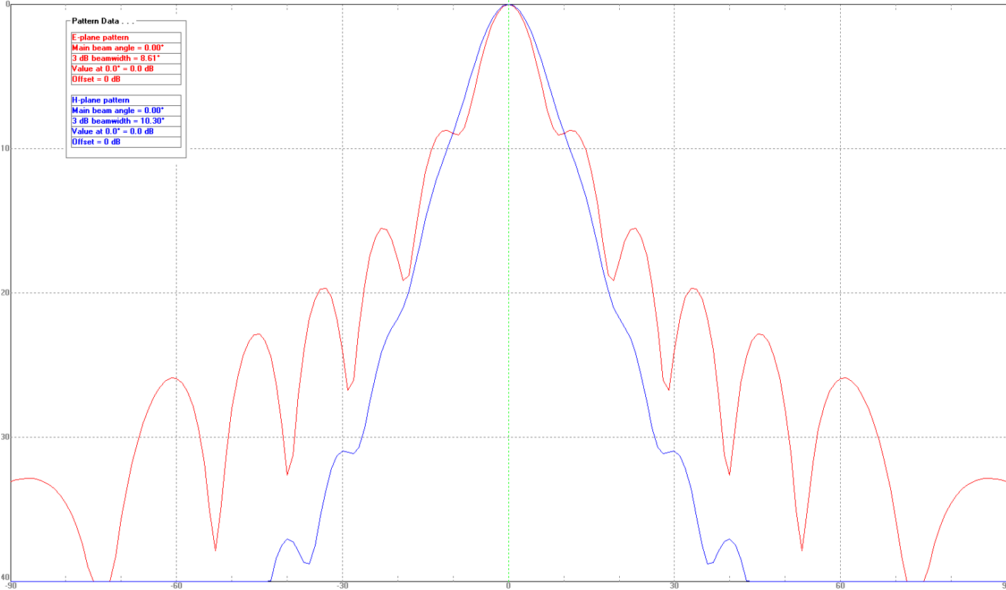
Beamwidth Pattern at 33.25 GHz
