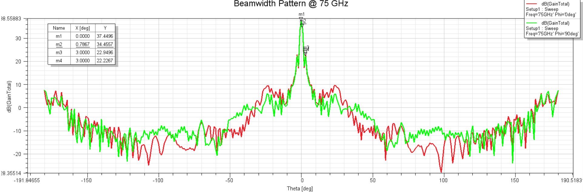
Beamwidth Pattern @ 75 GHz
