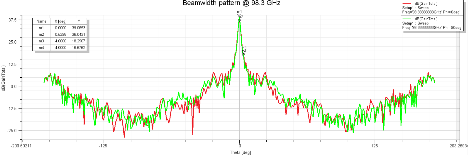
Beamwidth pattern @ 98.3 GHz
