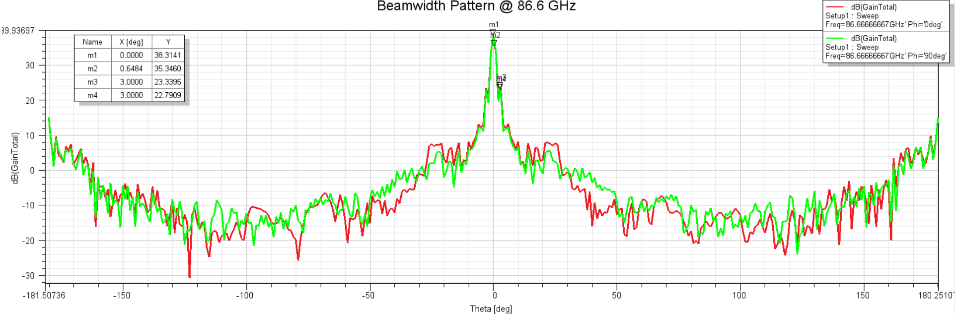
Beamwidth Pattern @ 86.6 GHz
