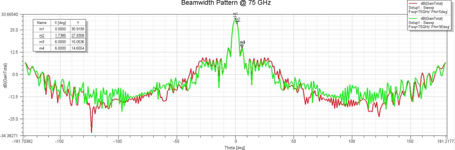
Beamwidth Pattern @ 75 GHz
