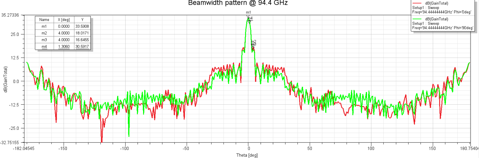
Beamwidth pattern @ 94.4 GHz
