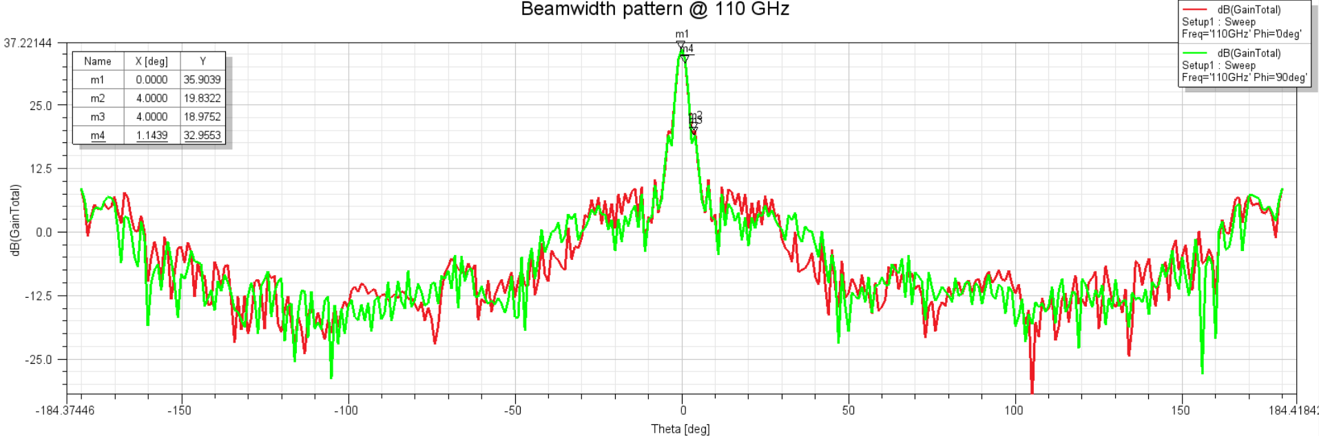
Beamwidth pattern @ 110 GHz
