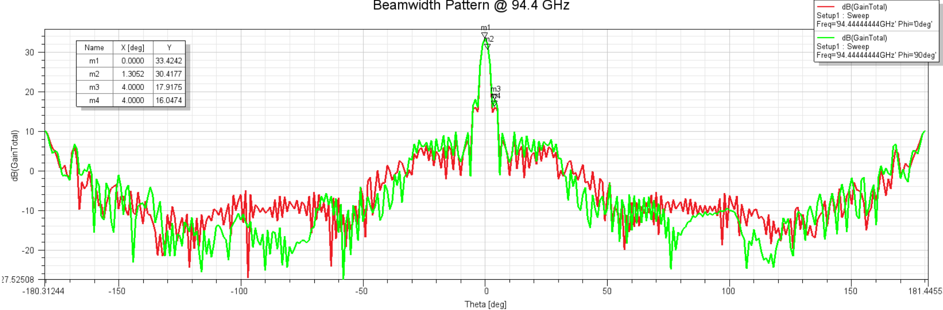
Beamwidth Pattern @ 94.4 GHz
