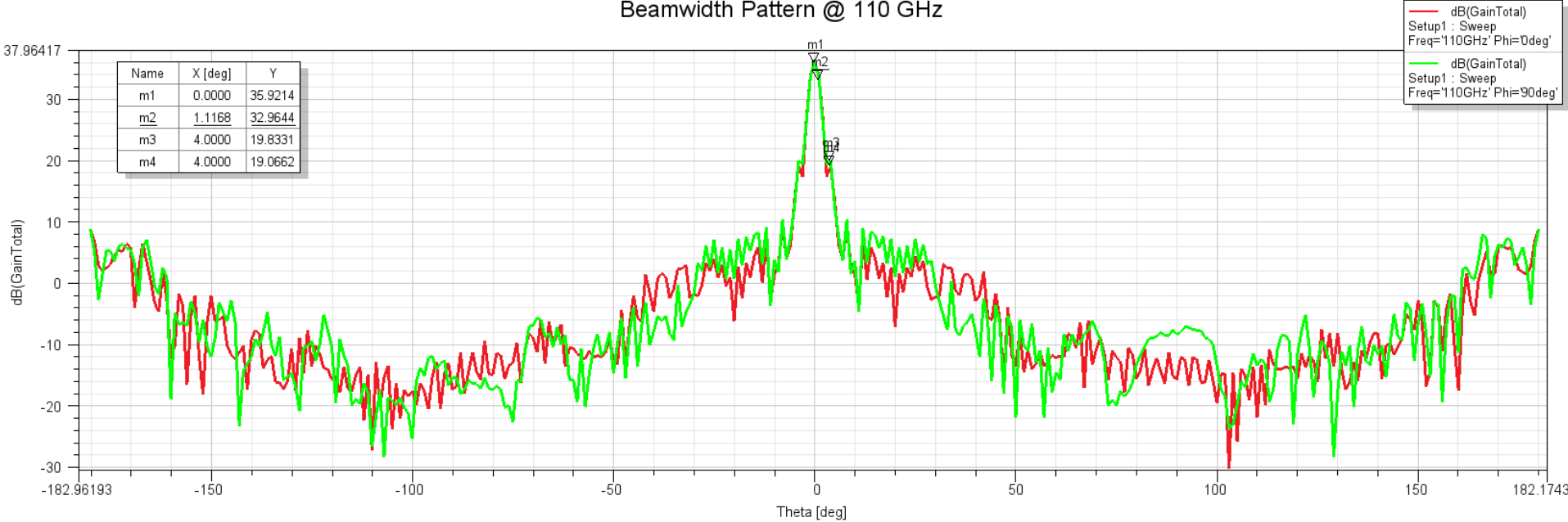
Beamwidth Pattern @ 110 GHz
