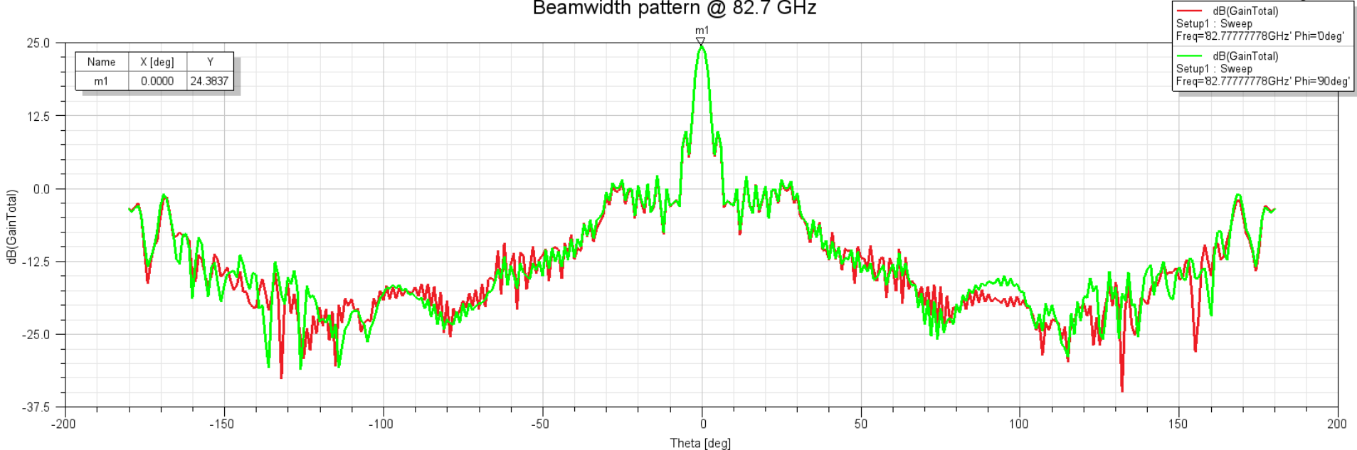
Beamwidth pattern @ 82.7 GHz
