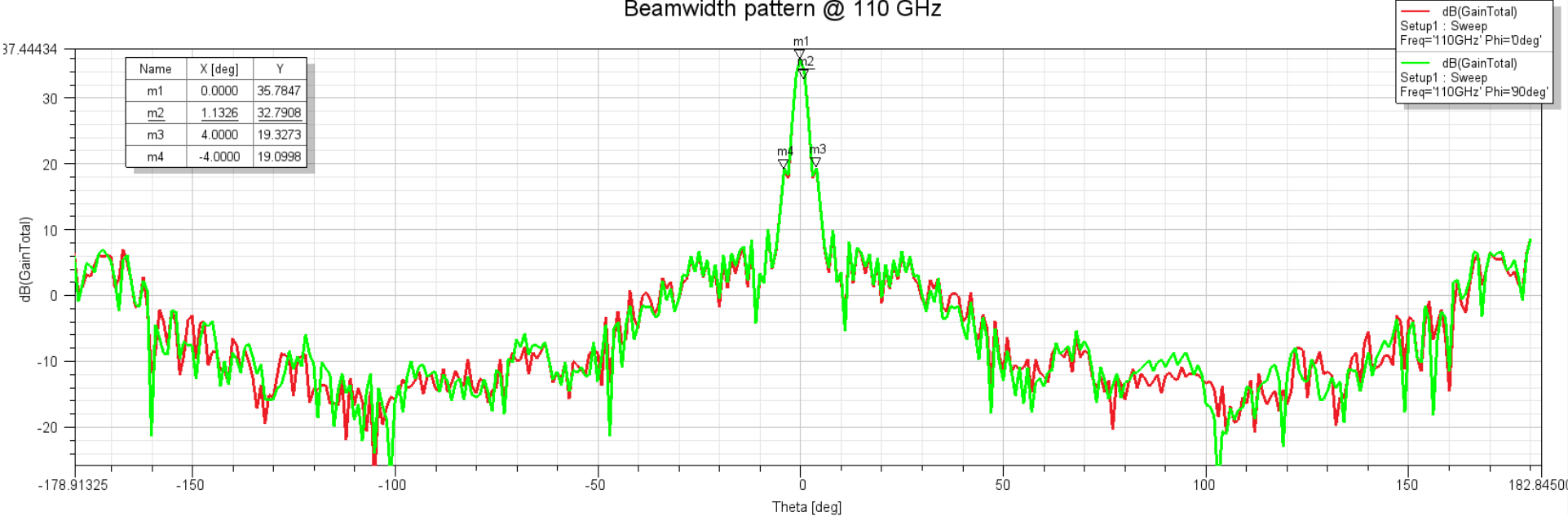
Beamwidth pattern @ 110 GHz
