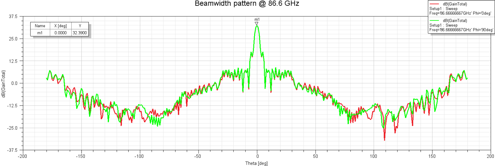
Beamwidth pattern @ 86.6 GHz
