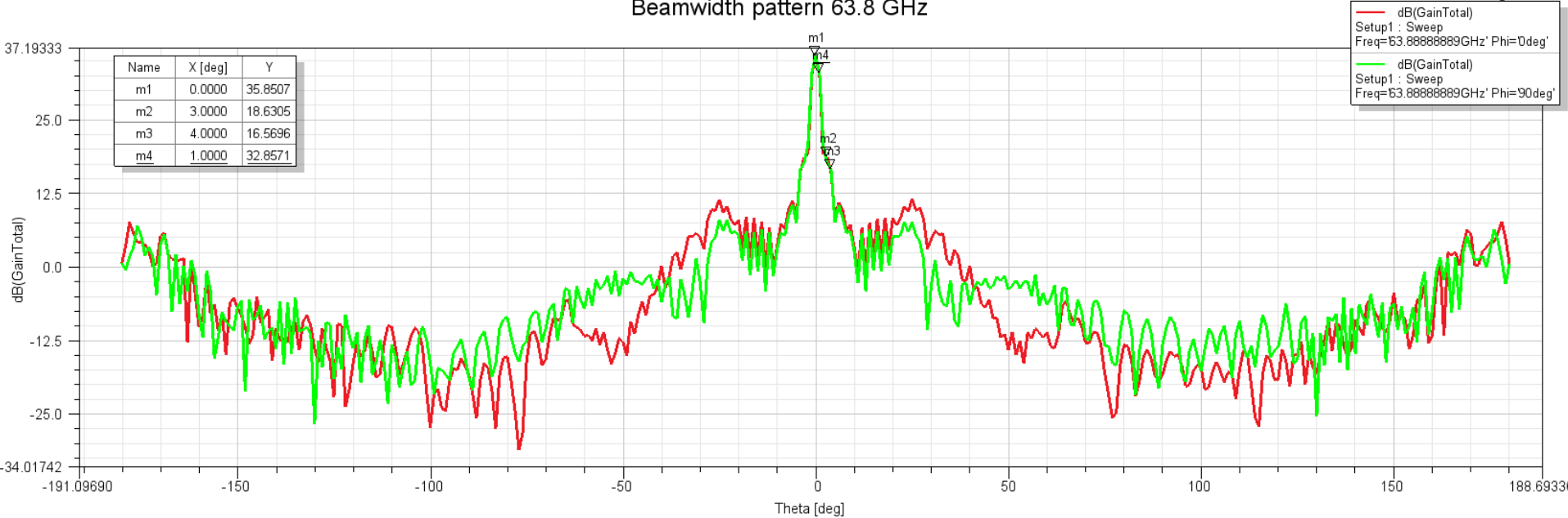
Beamwidth pattern 63.8 GHz
