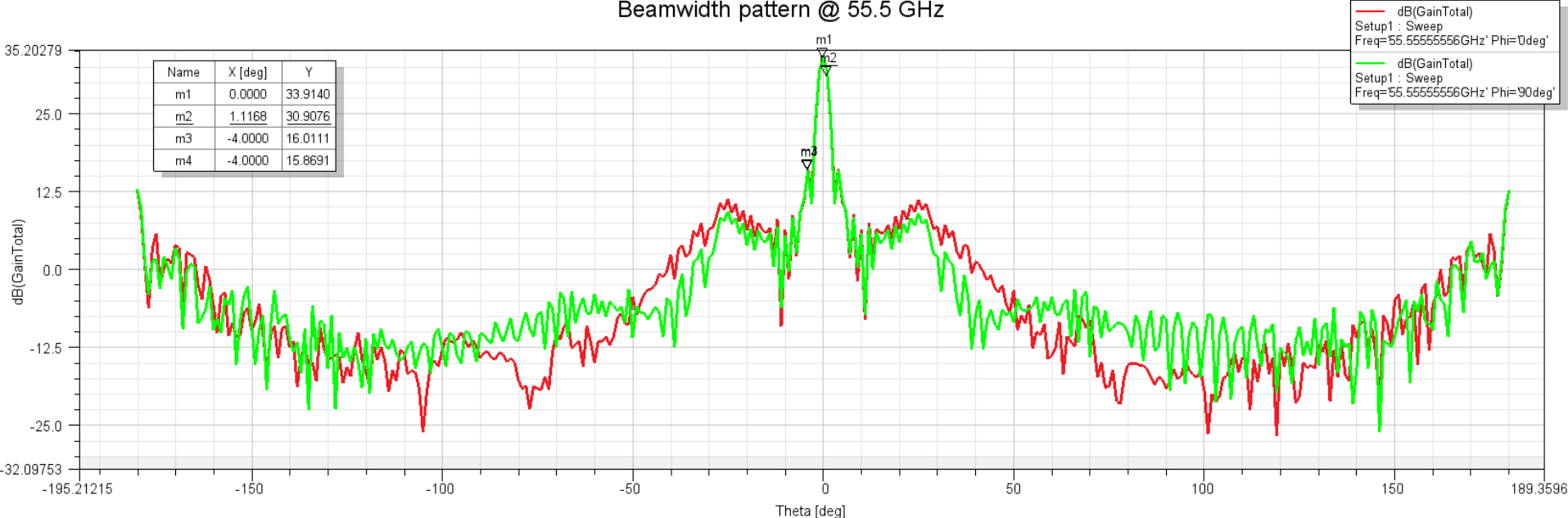
Beamwidth pattern @ 55.5 GHz
