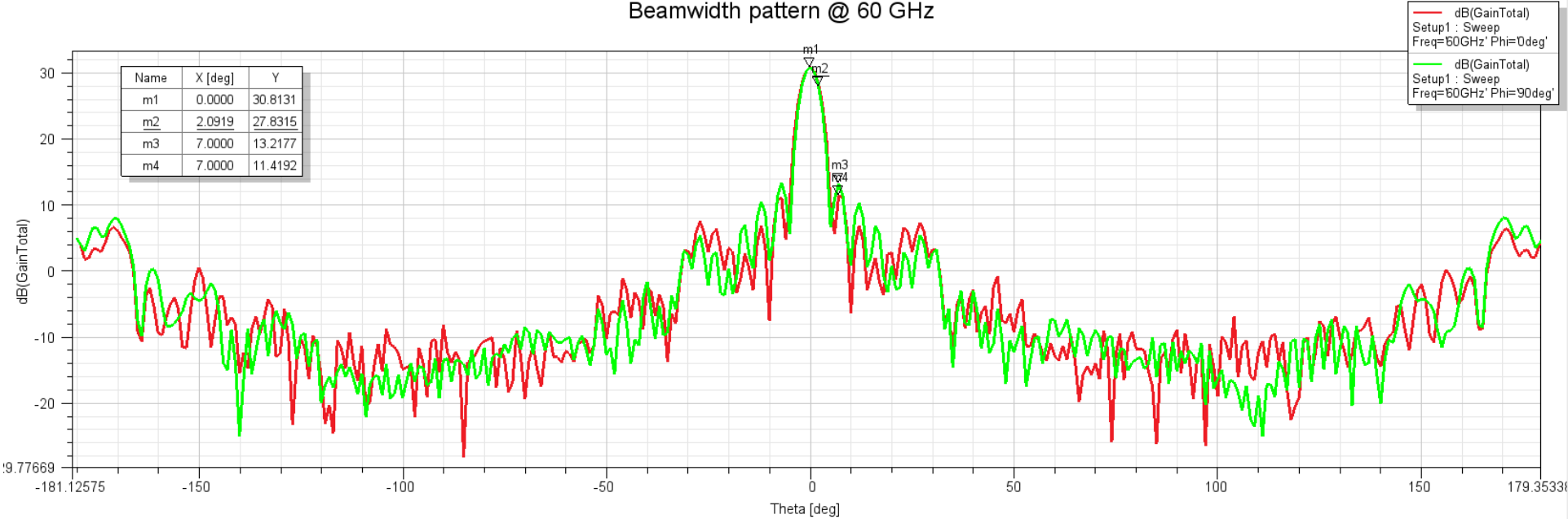
Beamwidth pattern @ 60 GHz
