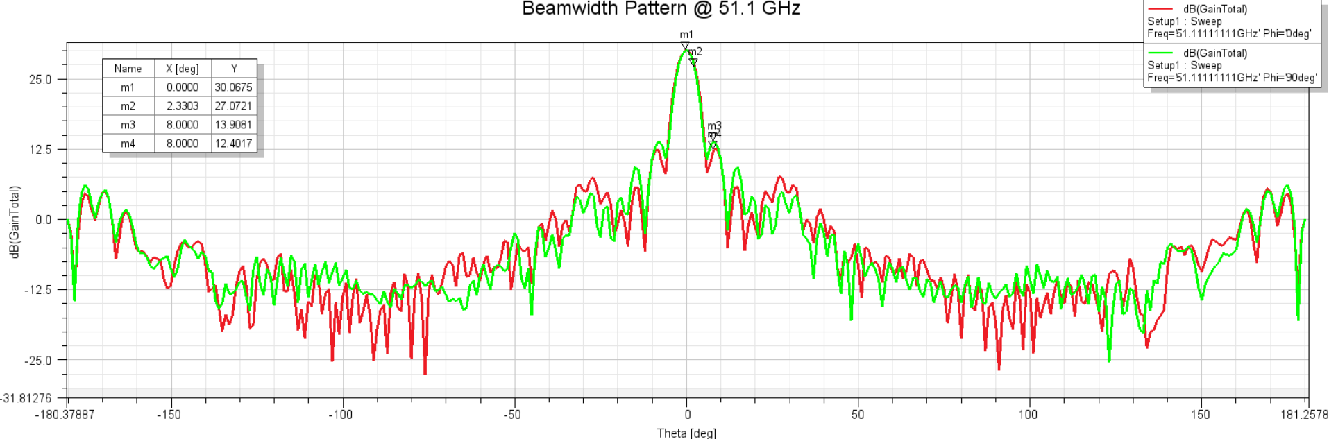
Beamwidth Pattern @ 51.1 GHz
