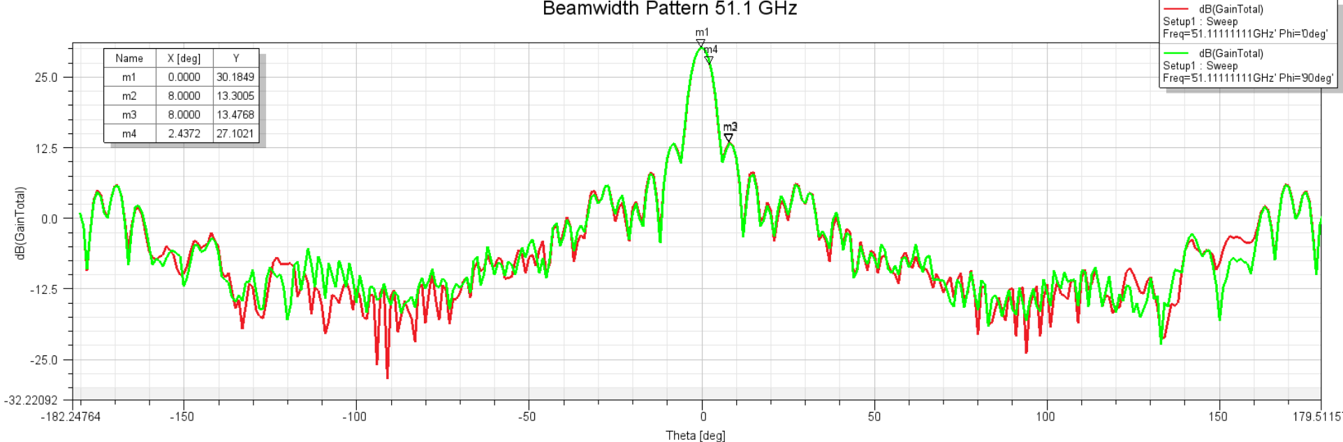
Beamwidth Pattern 51.1 GHz
