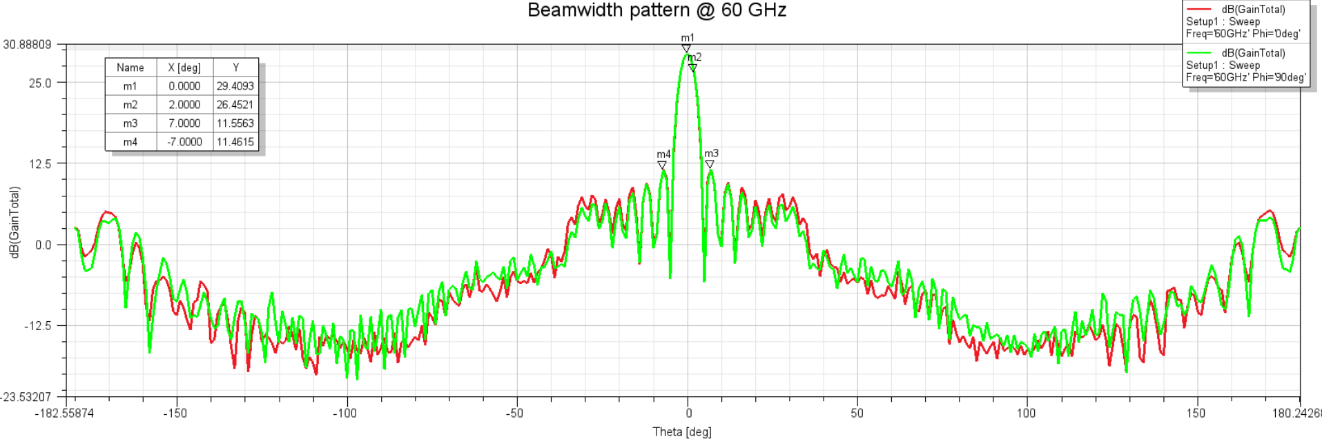
Beamwidth pattern @ 60 GHz
