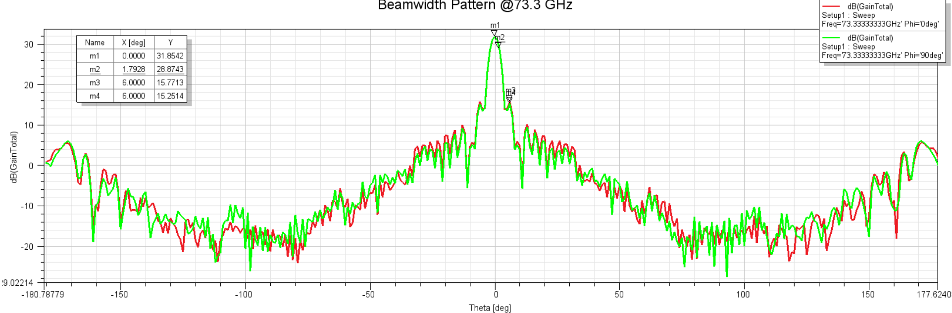
Beamwidth Pattern @73.3 GHz
