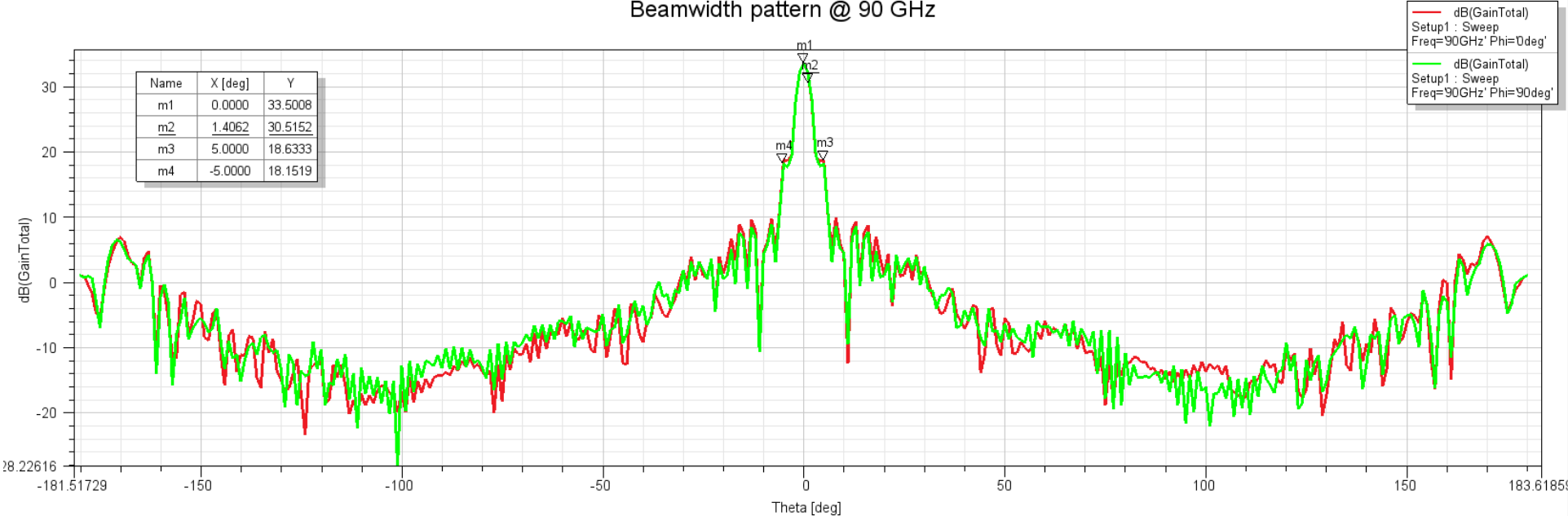
Beamwidth pattern @ 90 GHz
