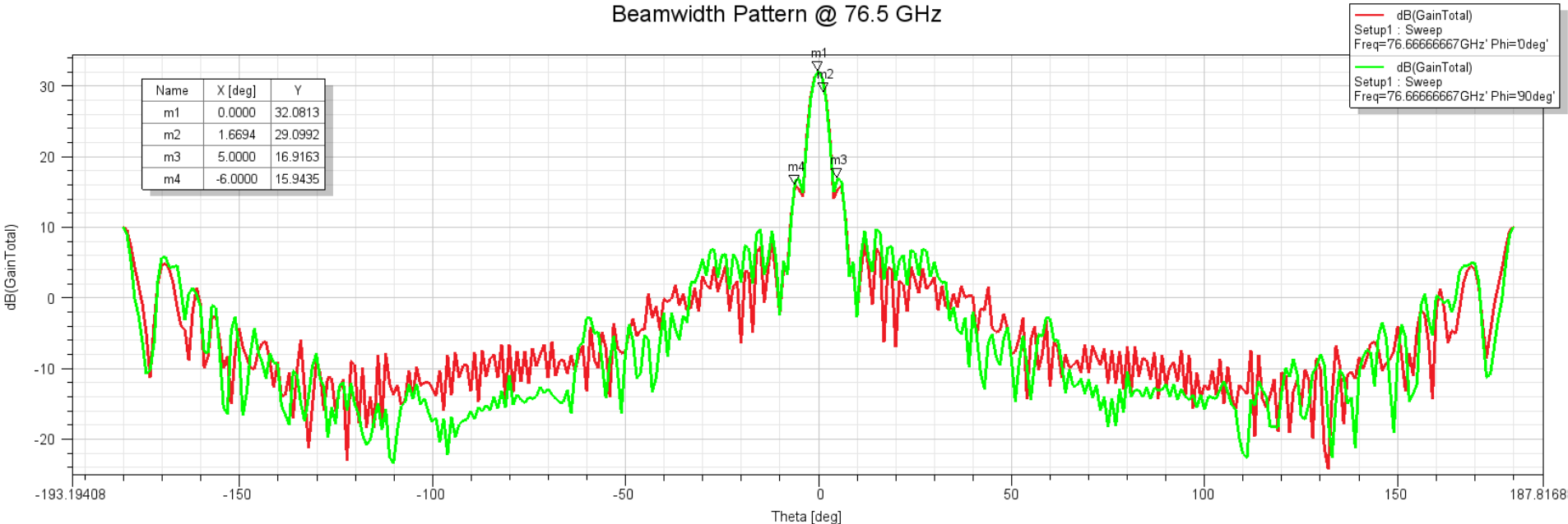
Beamwidth Pattern @ 76.5 GHz
