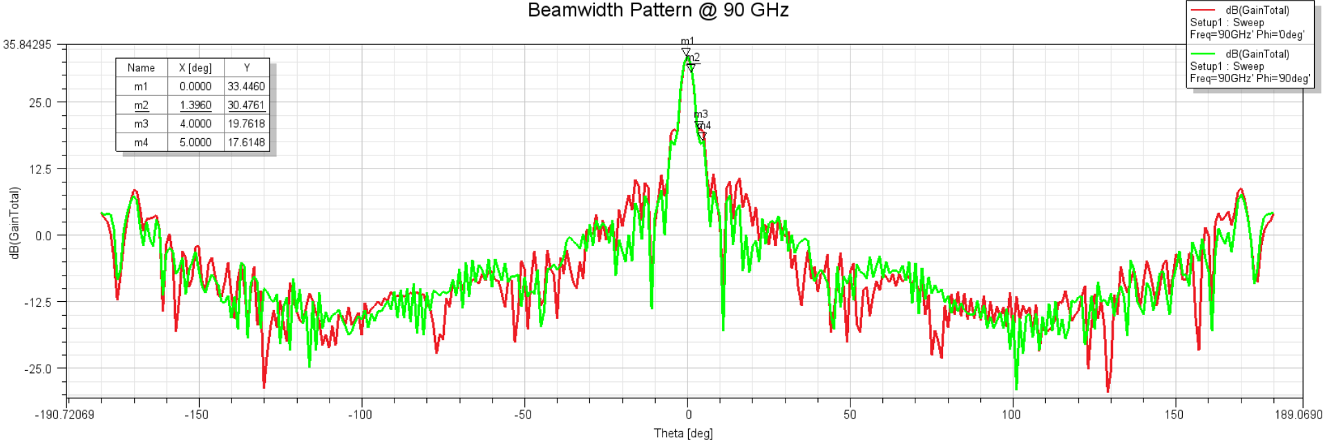
Beamwidth Pattern @ 90 GHz
