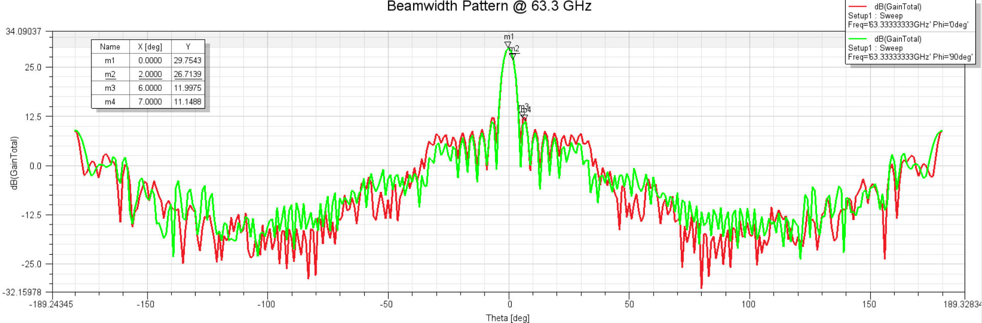
Beamwidth Pattern @ 63.3 GHz
