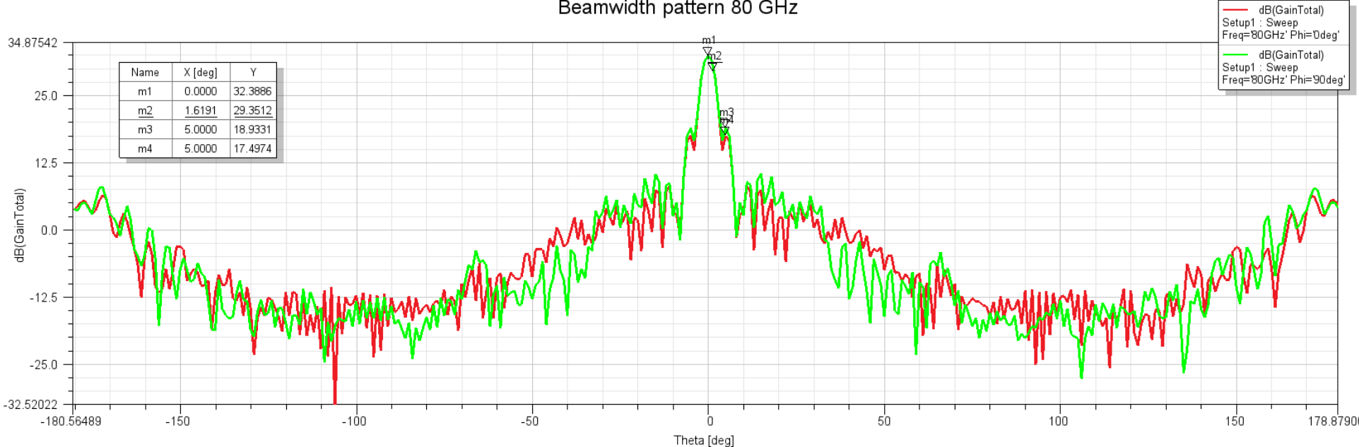
Beamwidth pattern 80 GHz
