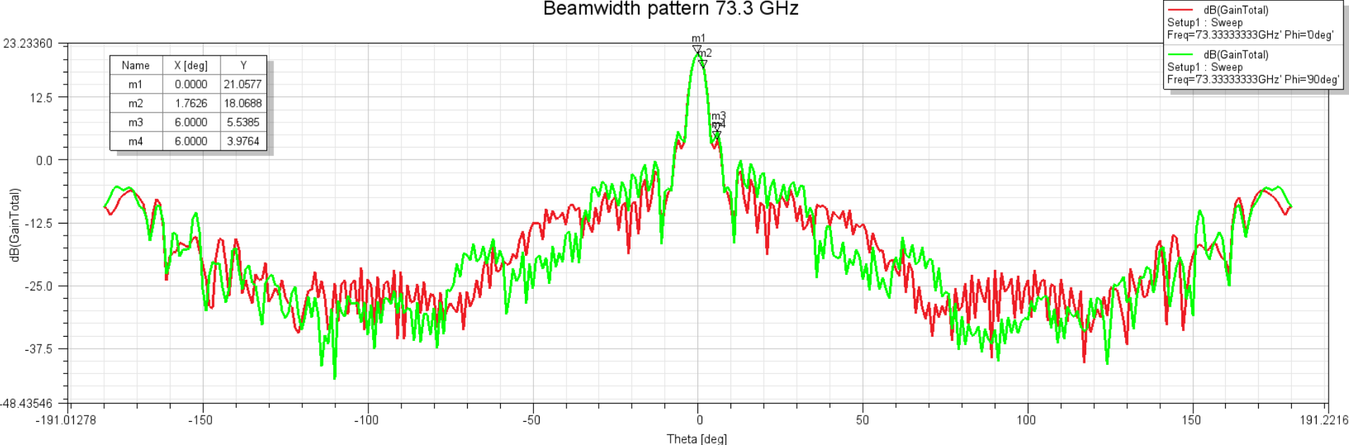
Beamwidth pattern 73.3 GHz
