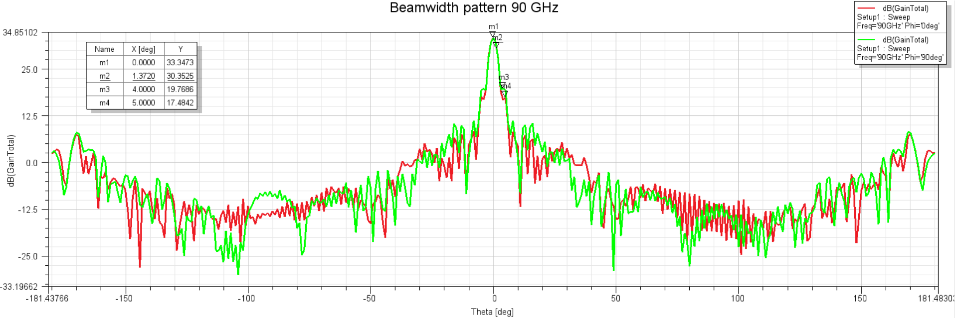
Beamwidth pattern 90 GHz
