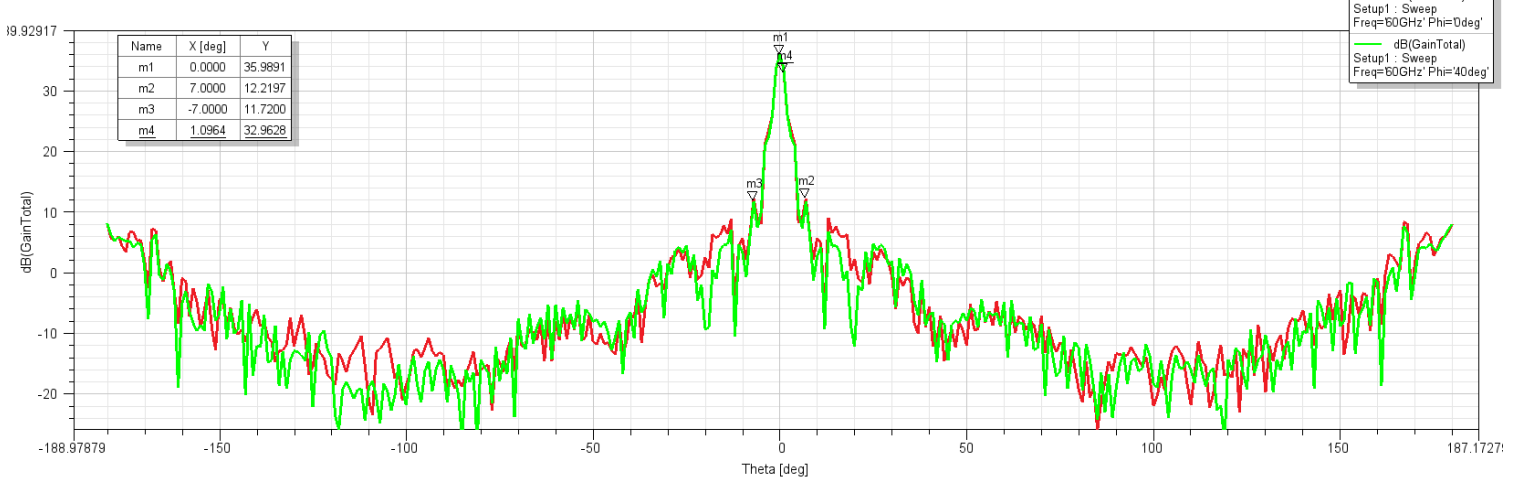
Beamwidth Pattern 60 GHz
