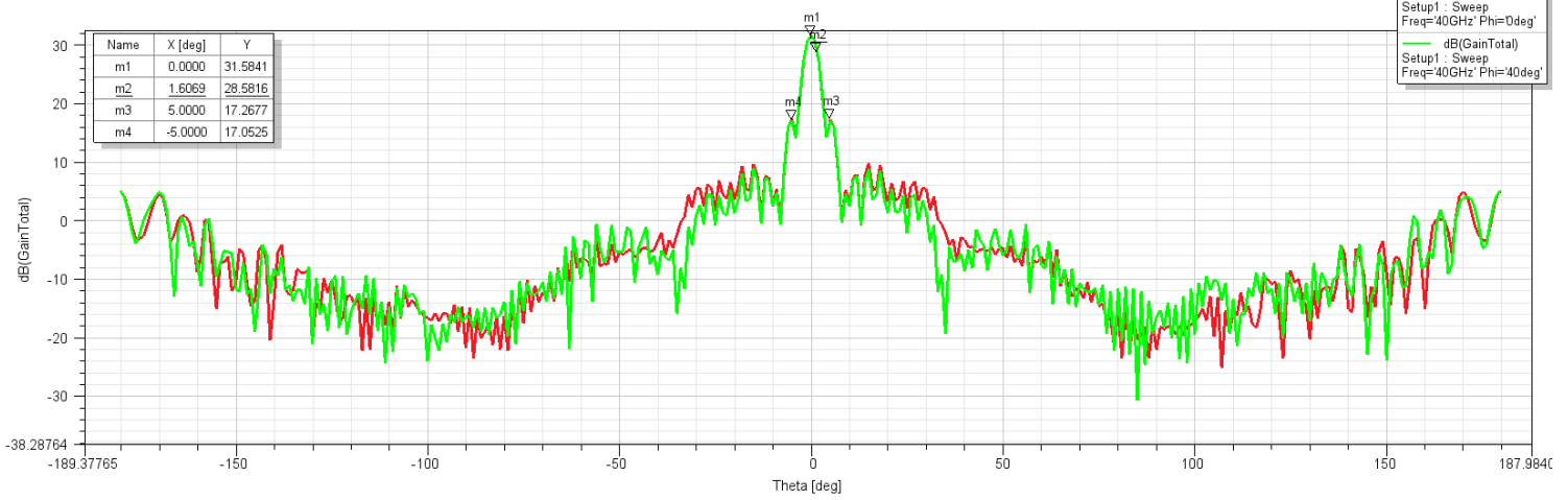
Beamwidth Pattern 51.1 GHz
