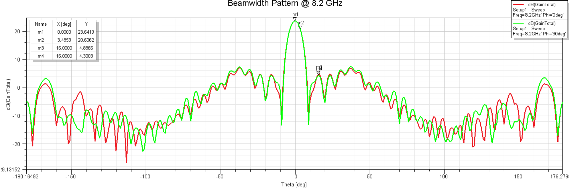
Beamwidth Pattern @ 8.2 GHz
