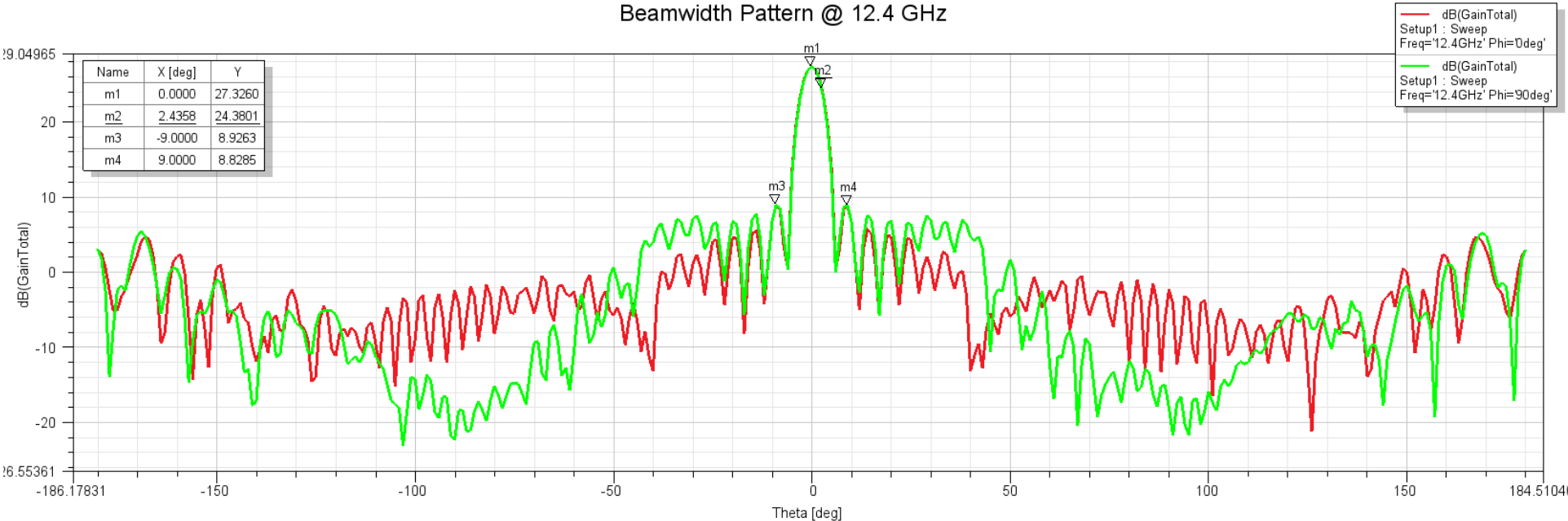
Beamwidth Pattern @ 12.4 GHz
