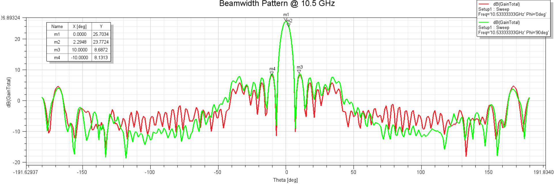
Beamwidth Pattern @ 10.5 GHz
