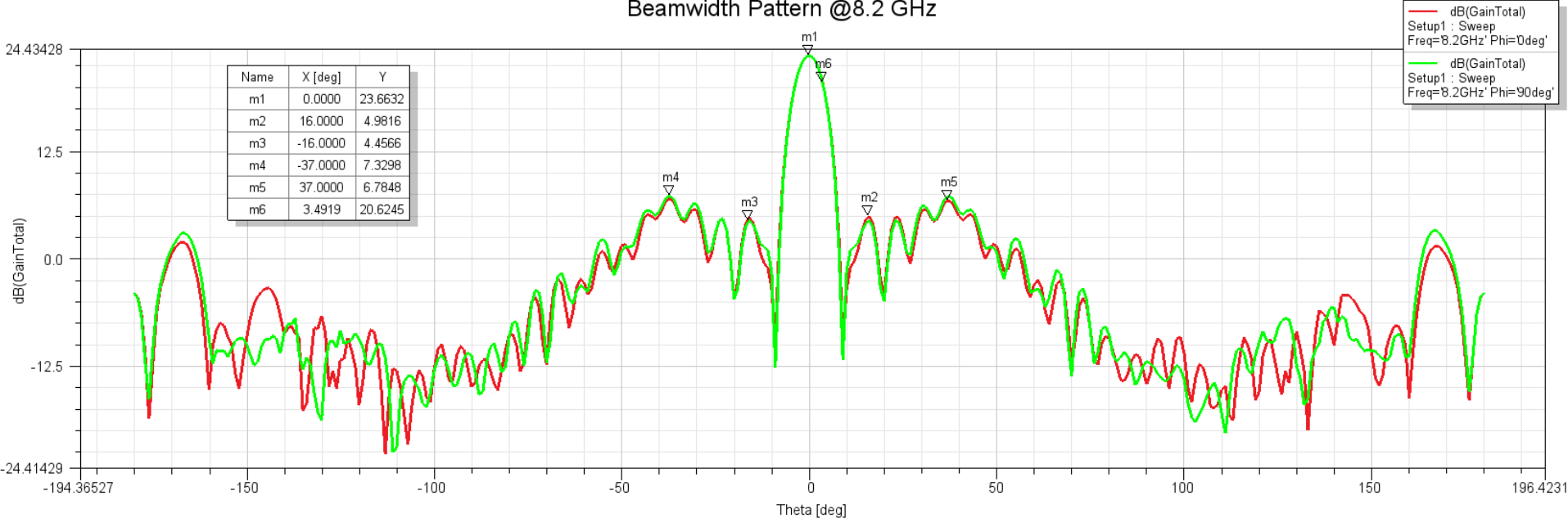
Beamwidth Pattern @8.2 GHz
