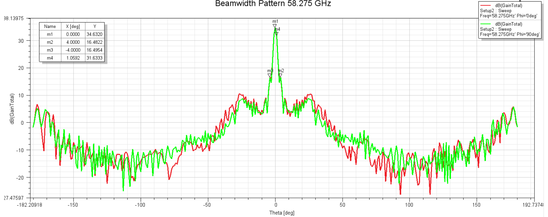
Beamwidth Pattern 58.275 GHz
