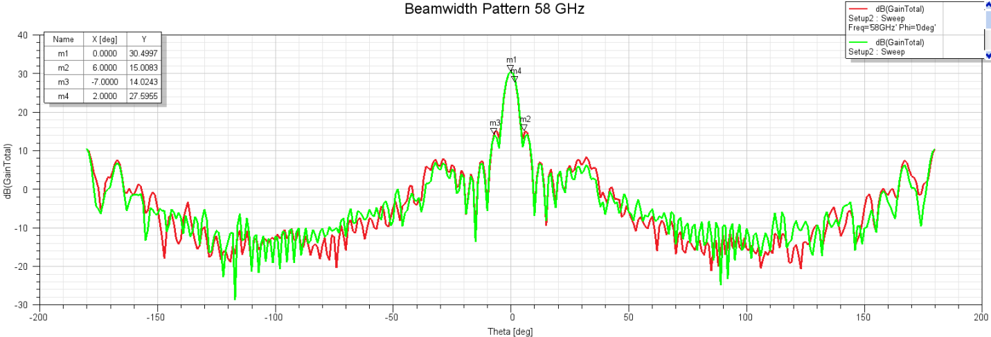
Beamwidth Pattern 58 GHz
