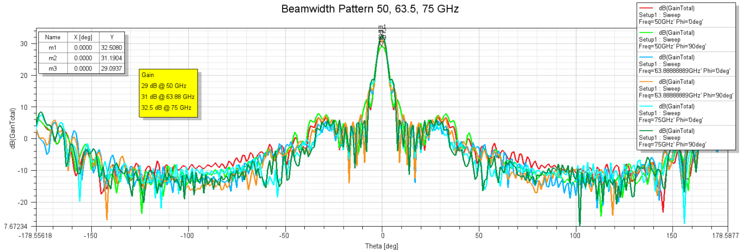
Beamwidth Pattern 50 GHz
