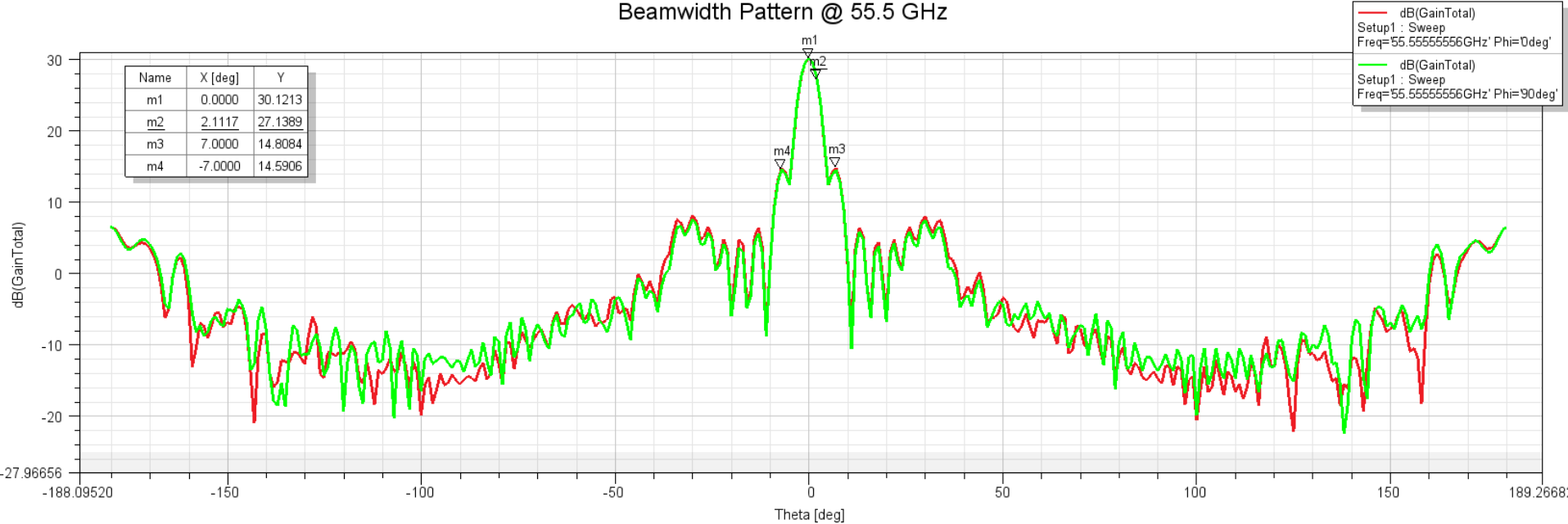
Beamwidth Pattern @ 55.5 GHz
