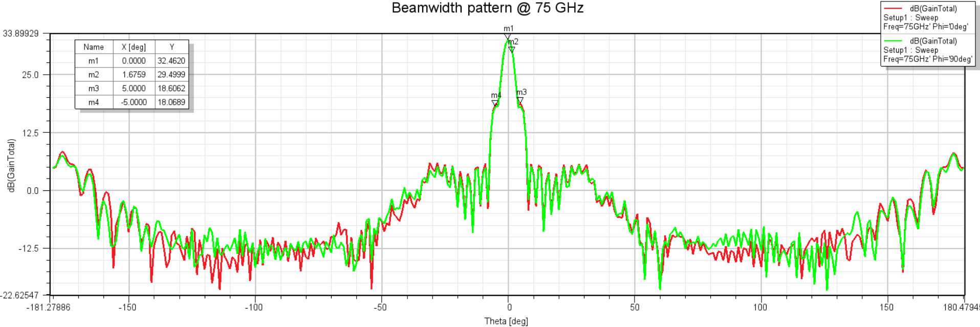
Beamwidth pattern @ 75 GHz
