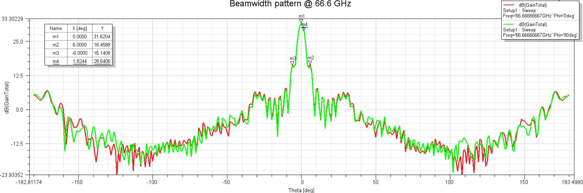
Beamwidth pattern @ 66.6 GHz
