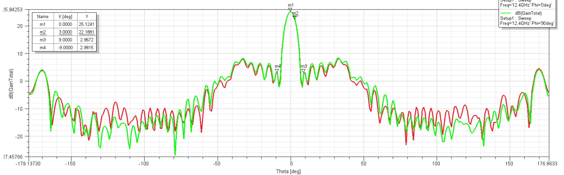
Beamwidth Pattern @ 15.5 GHz
