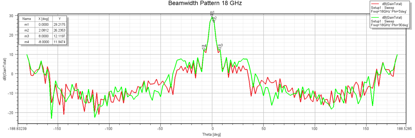
Beamwidth Pattern 18 GHz
