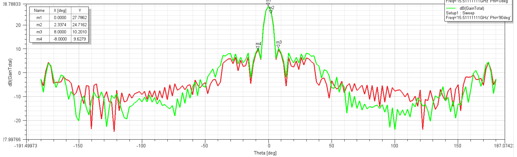
Beamwidth Pattern @ 15.5 GHz
