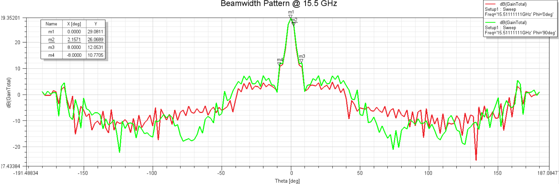
Beamwidth Pattern @ 15.5 GHz
