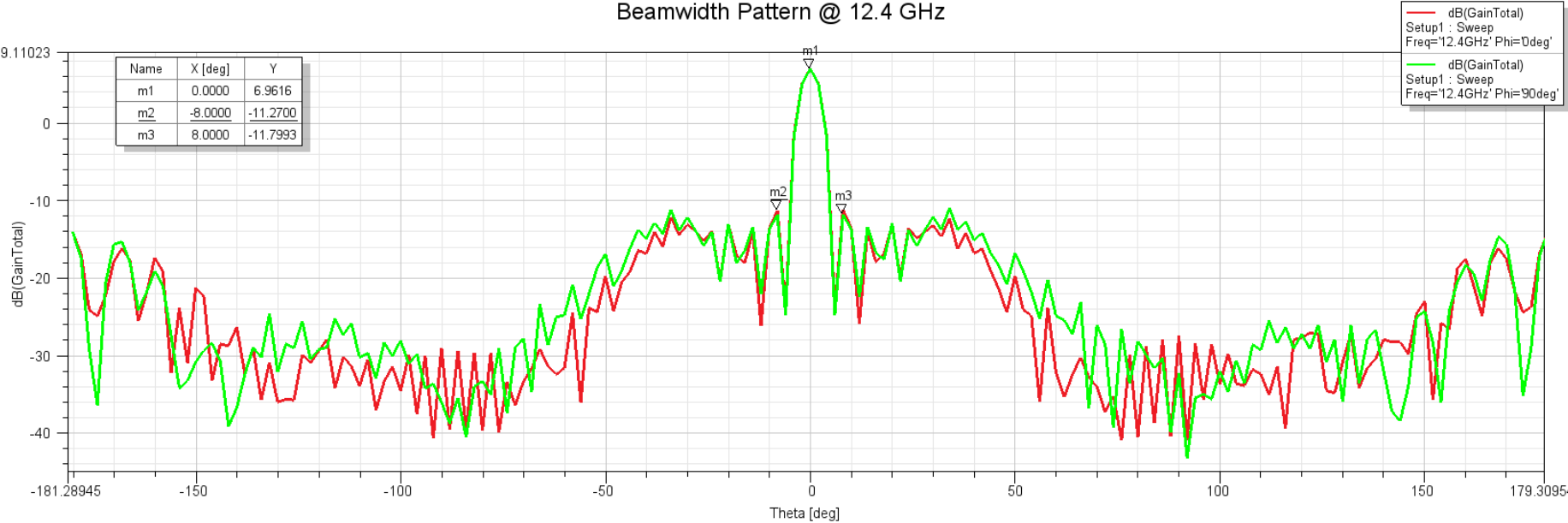
Beamwidth Pattern @ 12.4 GHz
