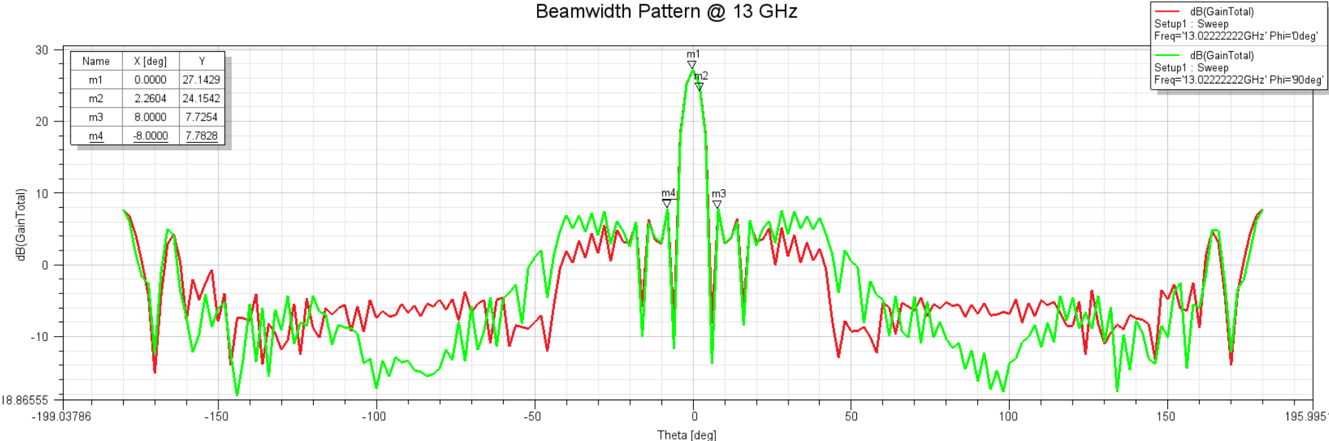
Beamwidth Pattern @ 13 GHz
