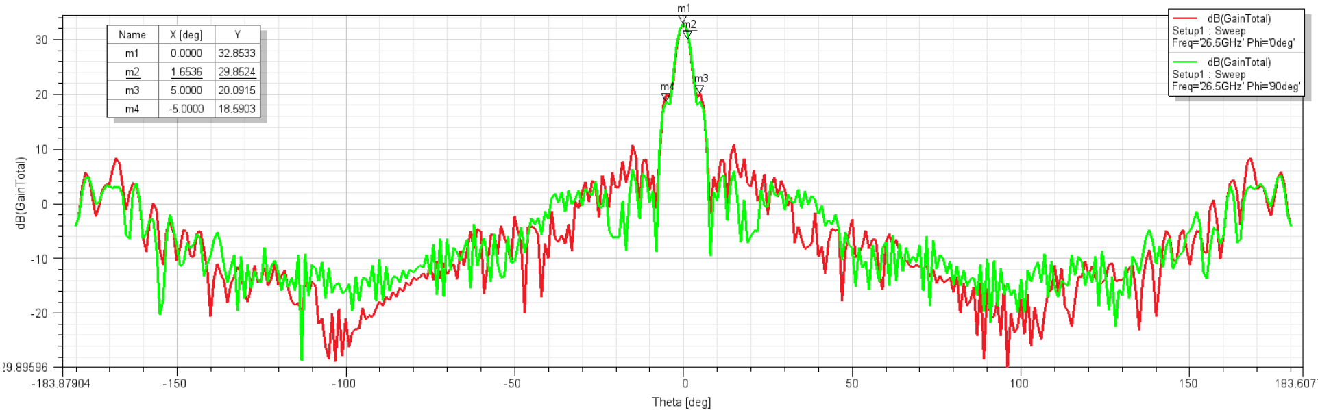
Beamwidth pattern @ 26.5 GHz
