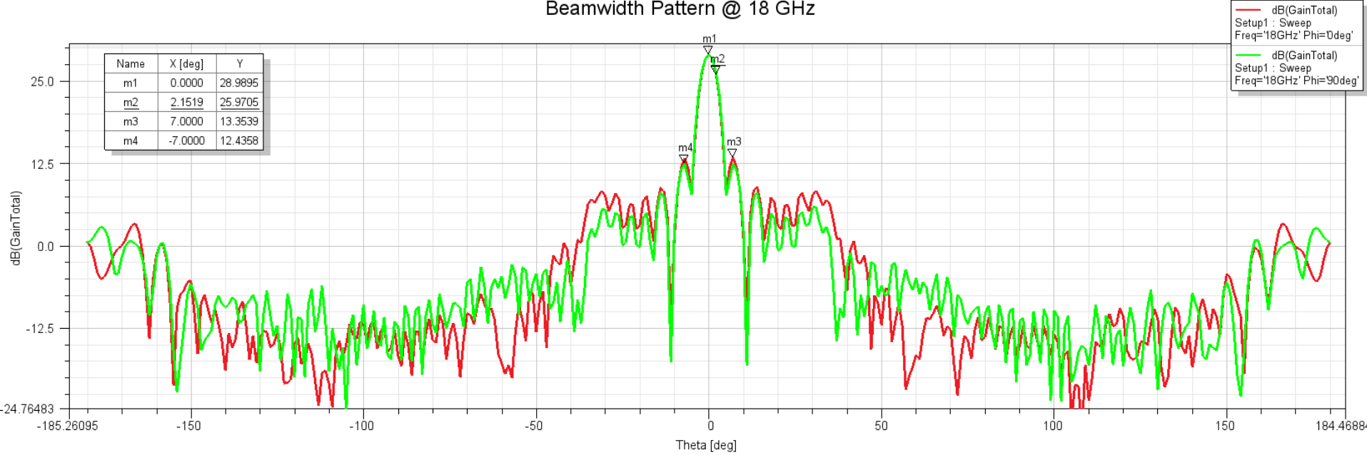
Beamwidth Pattern @ 18 GHz
