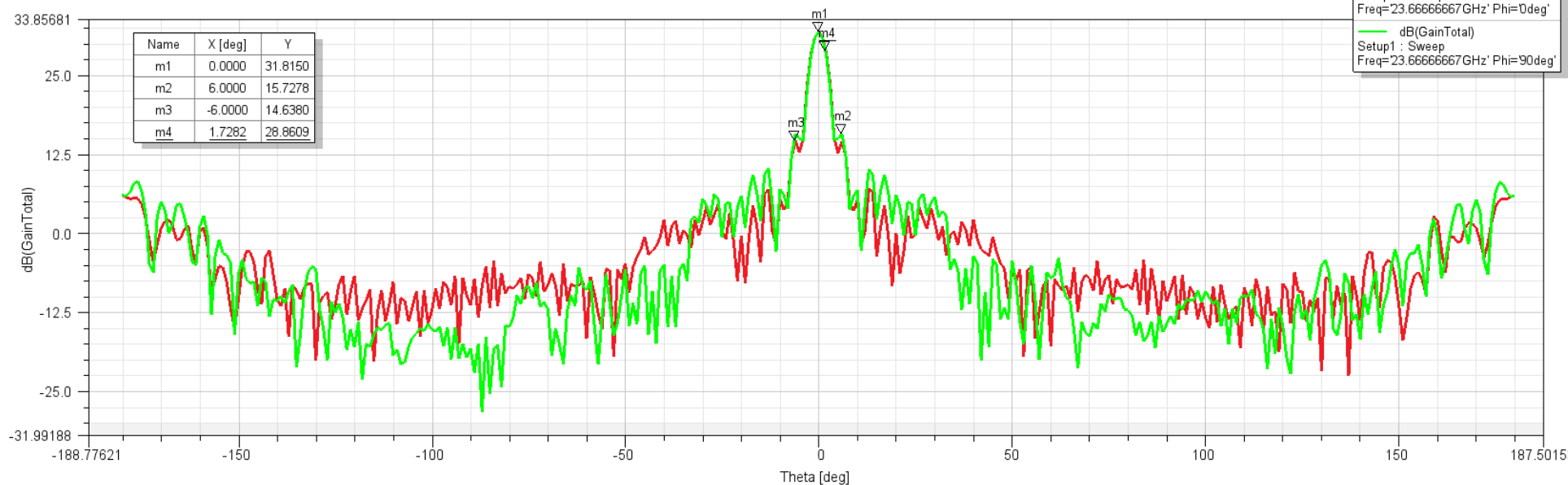
Beamwidth Pattern @ 23.6 GHz
