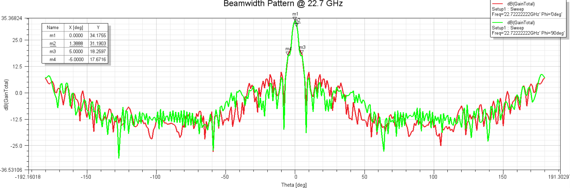
Beamwidth Pattern @ 22.7 GHz
