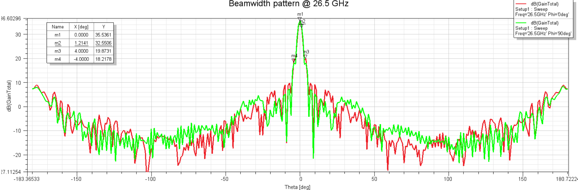
Beamwidth pattern @ 26.5 GHz
