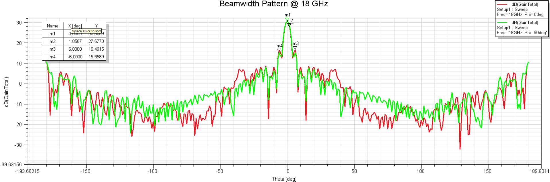
Beamwidth Pattern @ 18 GHz
