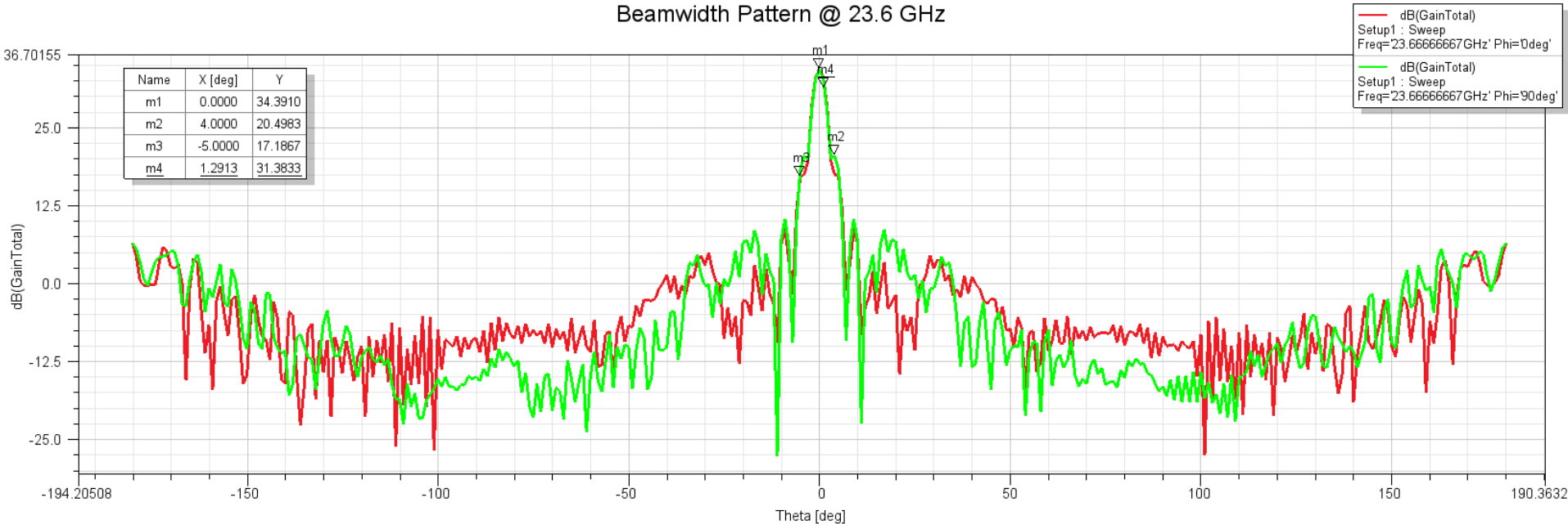
Beamwidth Pattern @ 23.6 GHz
