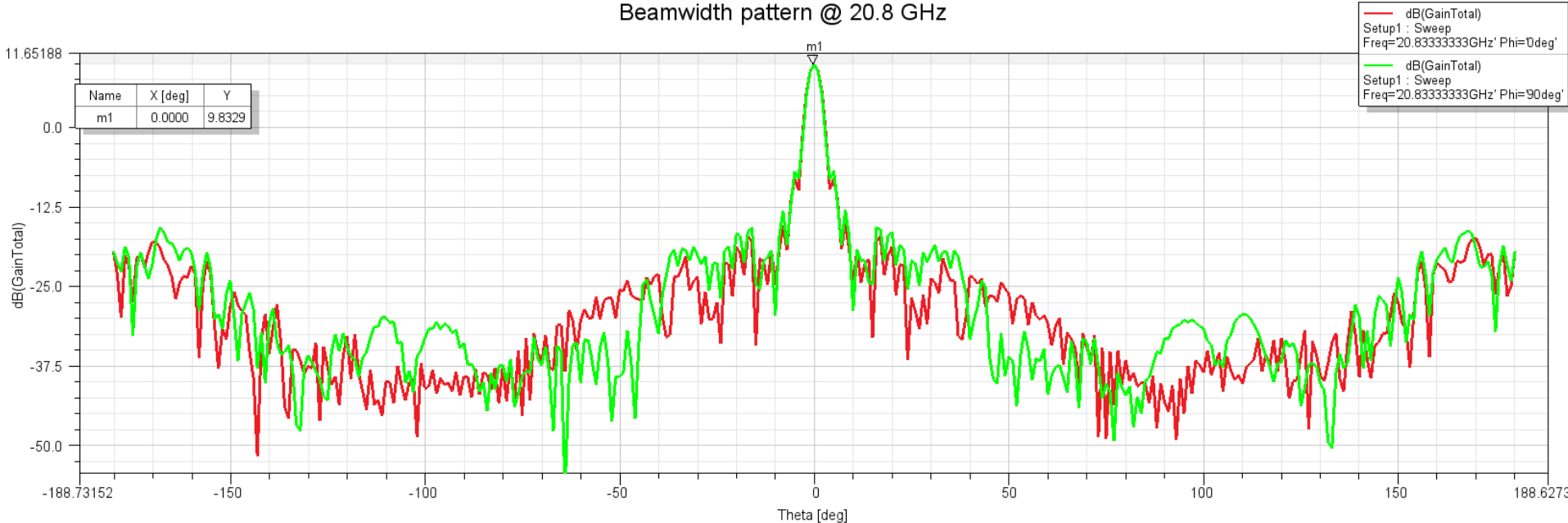
Beamwidth pattern @ 20.8 GHz
