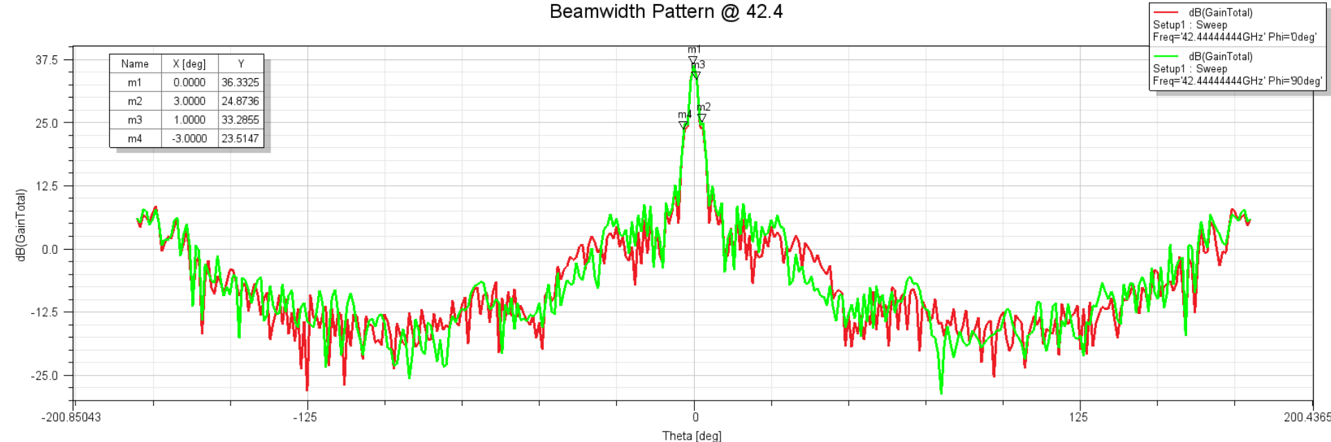
Beamwidth Pattern @ 42.4
