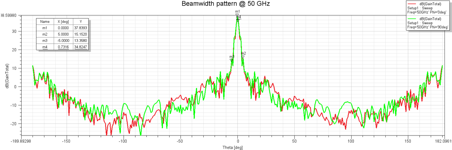
Beamwidth pattern @ 50 GHz
