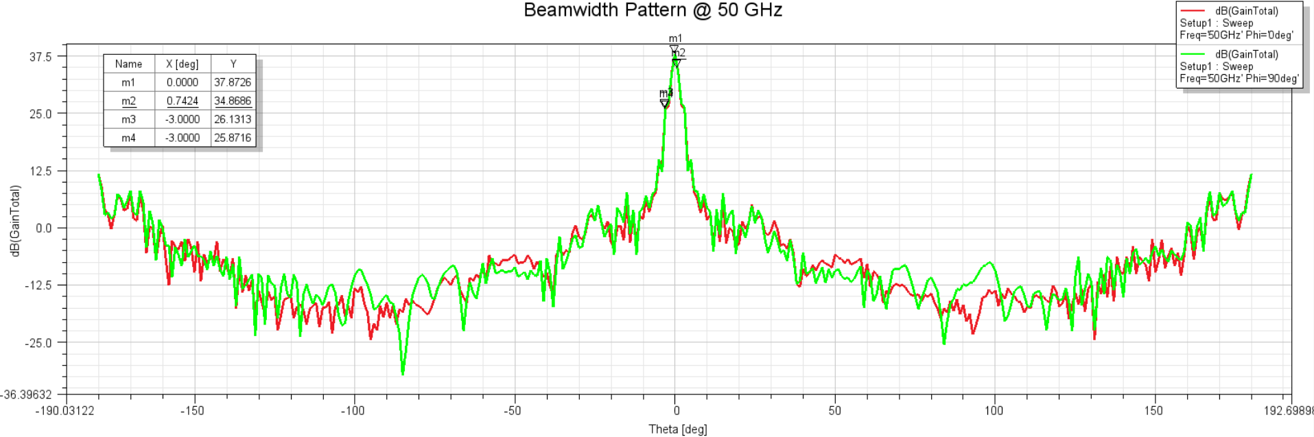
Beamwidth Pattern @ 50 GHz
