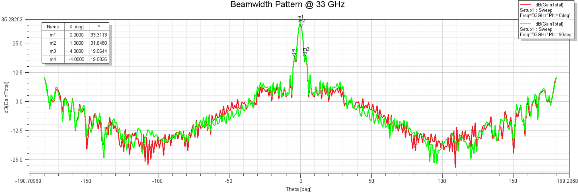
Beamwidth Pattern @ 33 GHz
