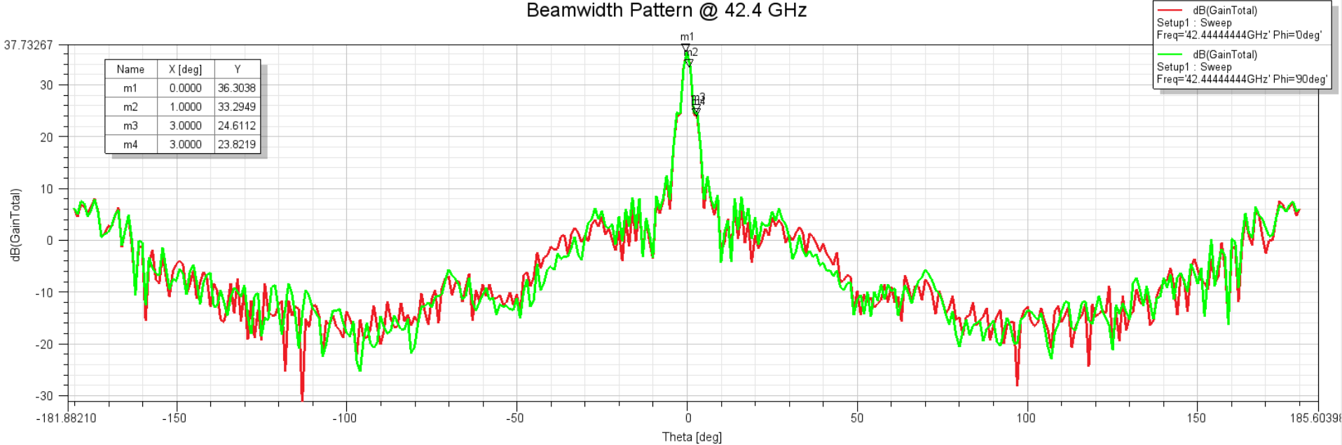
Beamwidth Pattern @ 42.4 GHz
