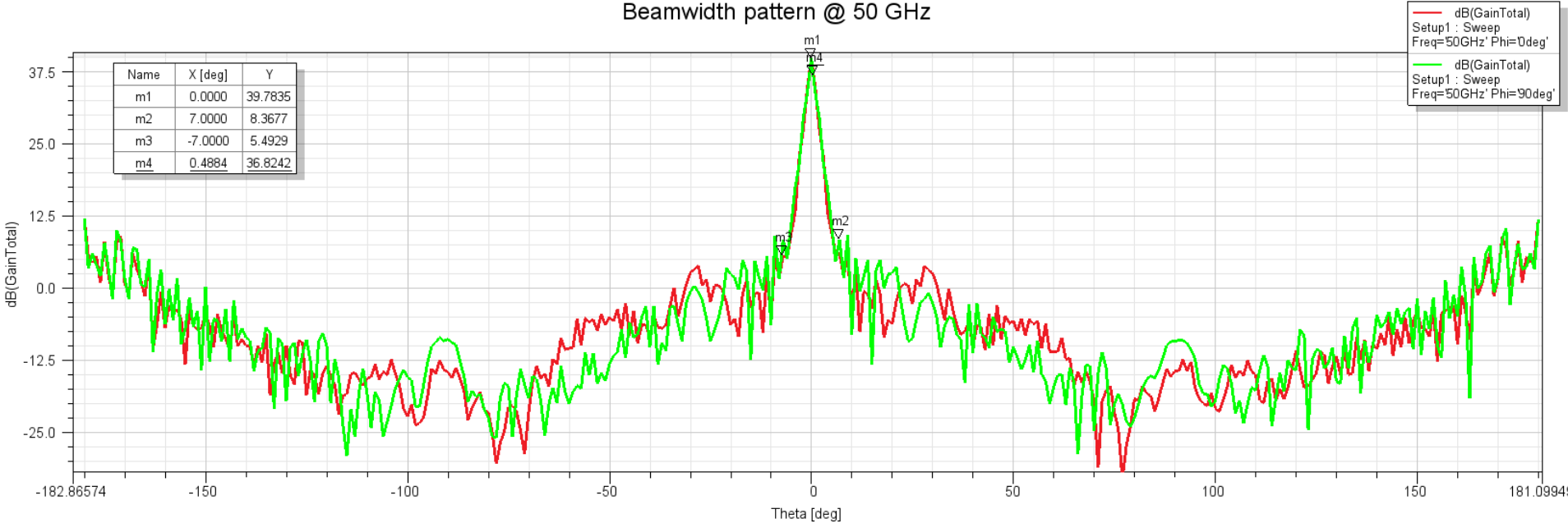
Beamwidth pattern @ 50 GHz
