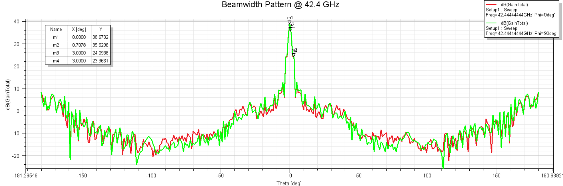
Beamwidth Pattern @ 42.4 GHz
