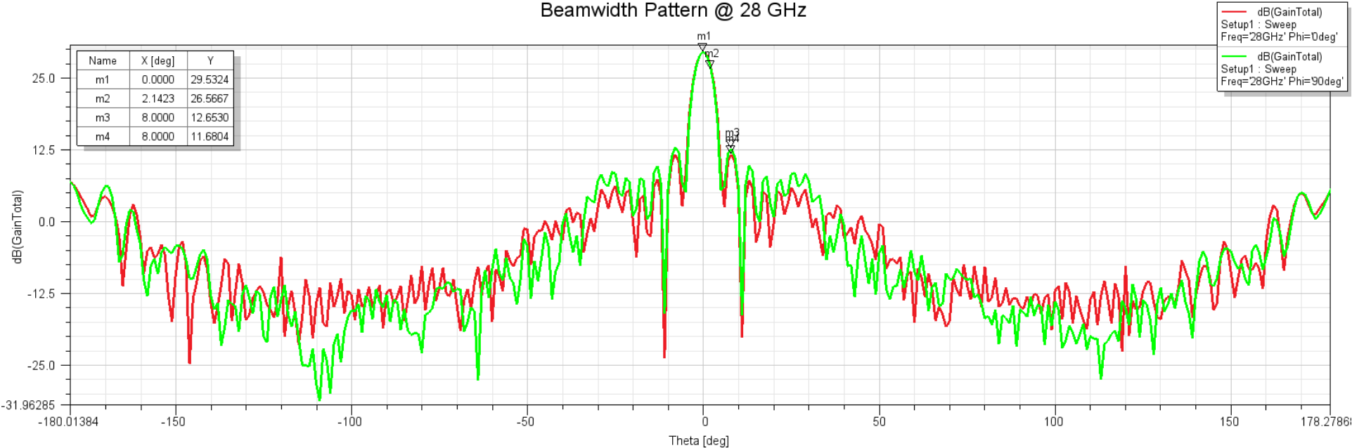
Beamwidth Pattern @ 28 GHz
