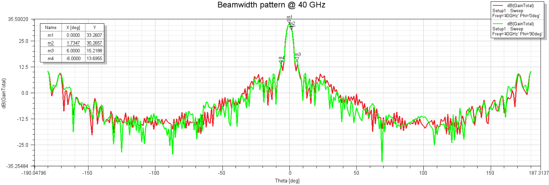
Beamwidth pattern @ 40 GHz
