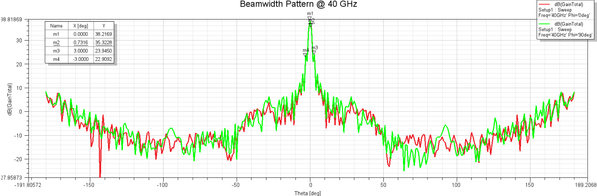
Beamwidth Pattern @ 40 GHz
