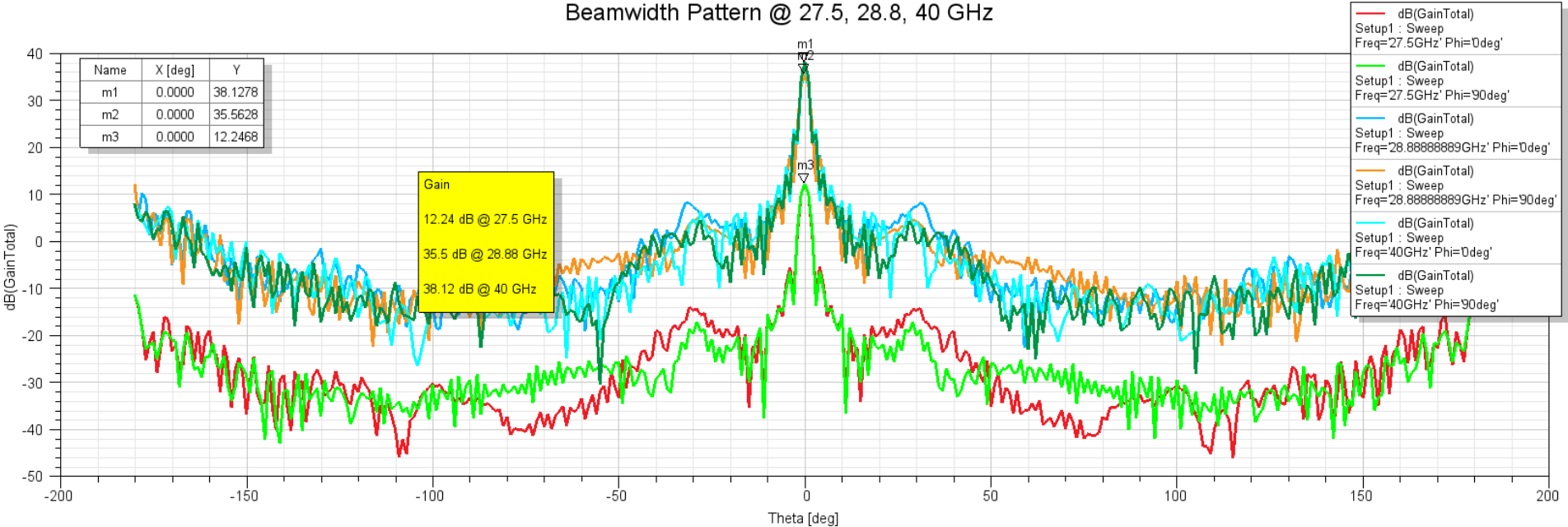
Beamwidth Pattern @ 27.5, 28.8, 40 GHz
