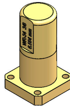
WR-34_WAVEGUIDE OFFSET
