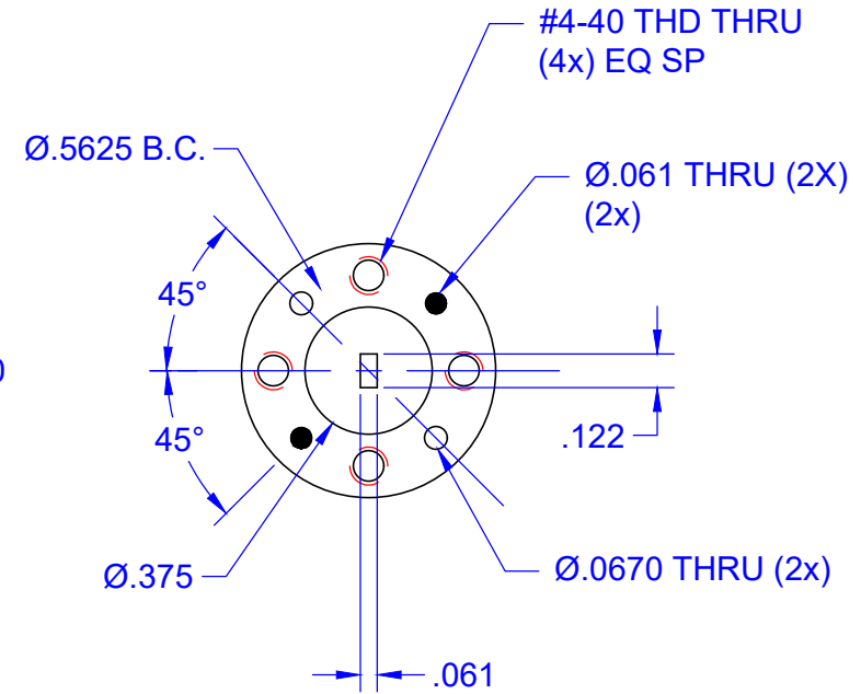
UG-387_FLANGE
