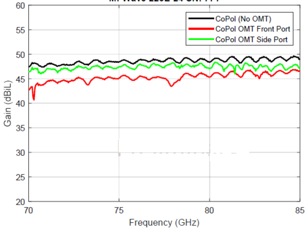
Measured Gain MI-Wave 223E-24 SN: 771
